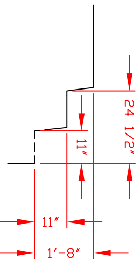
DETAIL 'A' FITTING FLAT
