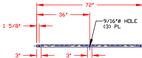
DETAIL ⑥ 1 1/2' X 1 1/2' X 3/16' ANGLE (4) REQ'D
