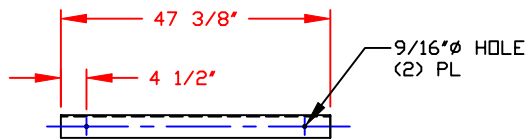
DETAIL ② 4' X 4' X 1/4' ANGLE (6) REQ'D
