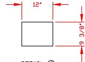
DETAIL ⑥ 1/8" THK X 12" FB (8) REQ'D SCALE: NONE
