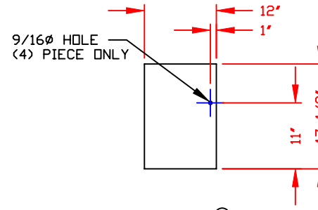
DETAIL ⑤ 3/16" THK X 12" FB (8) REQ'D (4) W/HOLES SCALE: NONE
