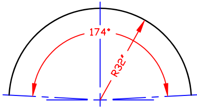
DETAIL ① 1/8" THK X 4" FLAT BAR ROLL TO 64" ID ARC LENGTH 97 3/8" (4) REQ'D
