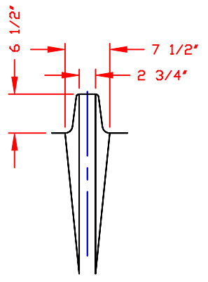
DETAIL 'D'
