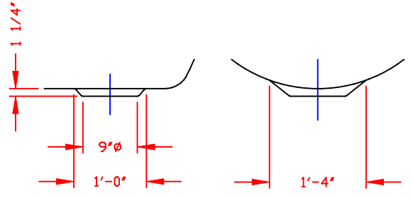
DETAIL 'C'
