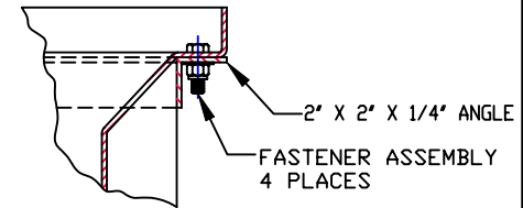
DETAIL "A" ANGLE ASSEMBLY STANDARD W/1.65 & 1.90 SpG TANKS. OPTIONAL W/1.35 SpG TANKS
