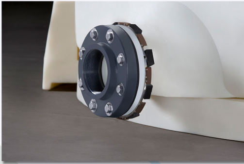
(IMFO™) Integrally Molded Full Discharge Tank
