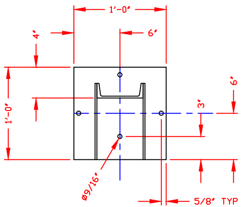
BASEPLATE DETAIL
