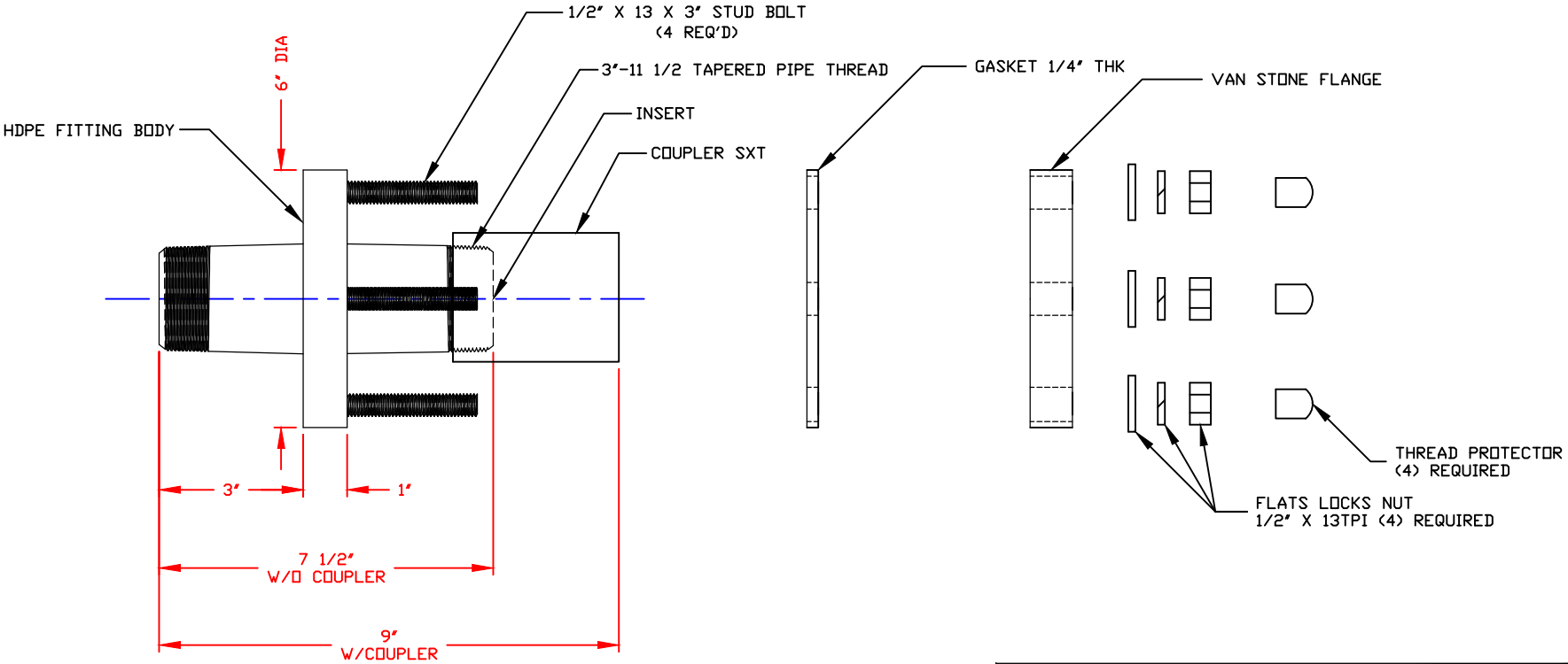
SIDE VIEW
