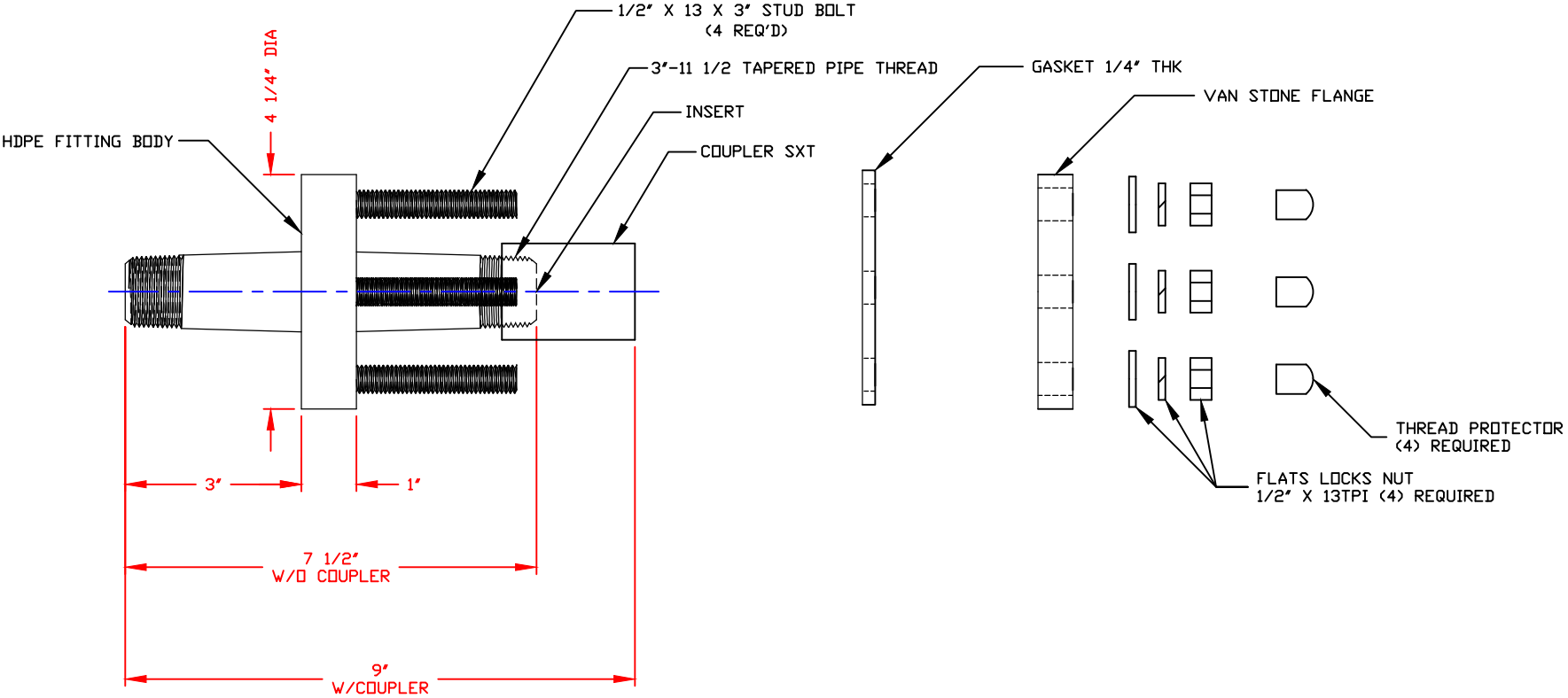
ELEVATION VIEW
