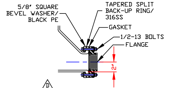
DETAIL "A" (INTEGRALLY MOLDED FLANGED OUTLET) AVAILABLE IN 4" SIZE ONLY SCALE: NONE
