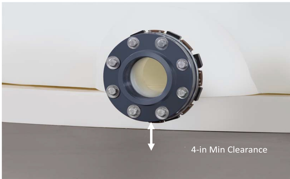
CORRECT STORAGE. Notice clearance of flange above the floor.
